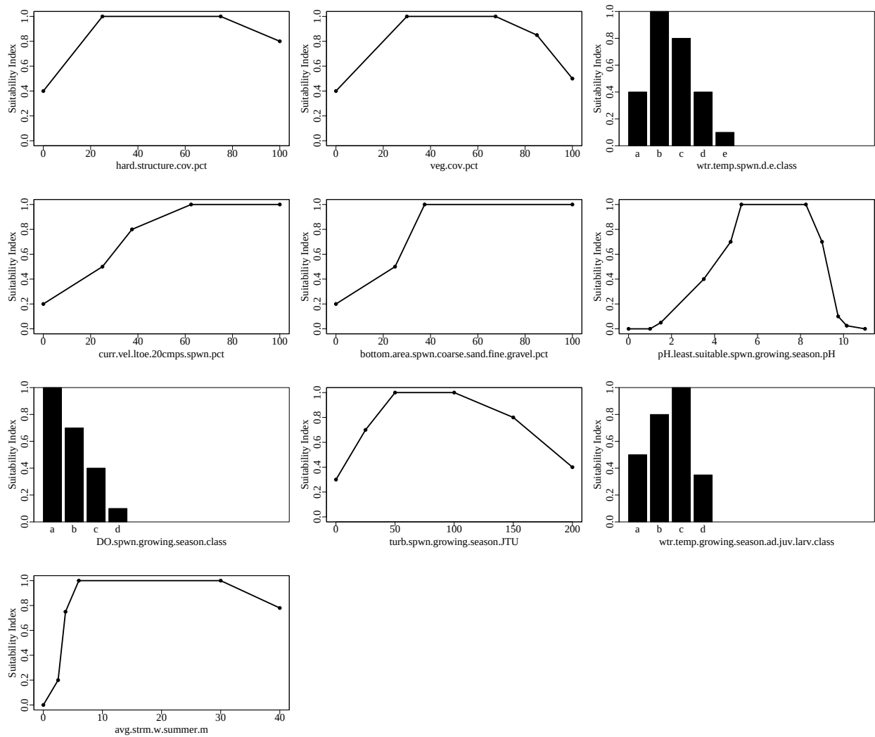
Figure 1. Suitability index graphs for variables included in the redbreastsunfishRiv model in ecoRest.
